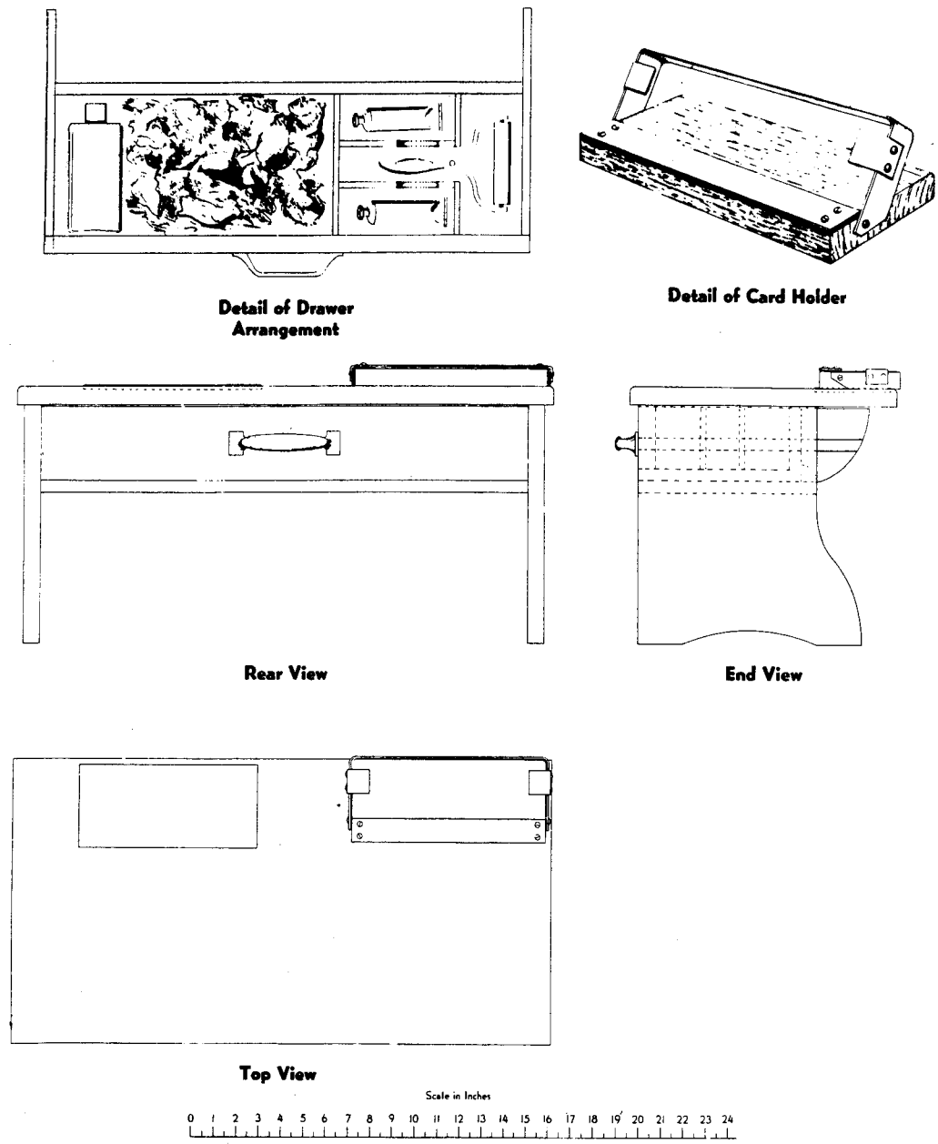
408. Diagram of a Fingerprint Inking Stand
