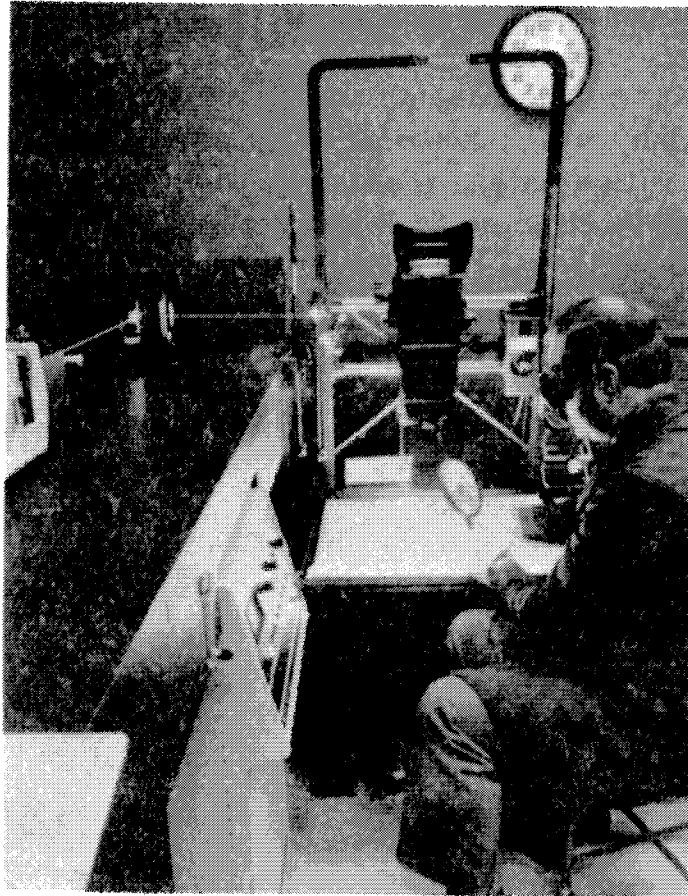
427. Detecting latent prints with 18 watt continuous wave argon ion laser.
